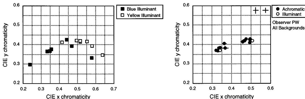
Fig. 6. Effect of background surface. The left panel shows the chromaticities of the Gray, Red, Yellow, Dark Blue, Brown, White, and Black background surfaces under the Blue and Yellow illuminants. Solid squares, chromaticities of the light reflected from the background surfaces under the Blue illuminant; open squares, corresponding chromaticities under the Yellow illuminant. The right panel shows the achromatic loci for observer PW measured for the seven background surfaces. Solid circles, achromatic loci; open circles, chromaticities of the Blue and Yellow illuminants. The error bars on the solid circles represent \pm 1 between-session standard error. Note that the achromatic loci cluster near the illuminant even though the chromaticities of the background surfaces scatter widely. For each condition, we computed the average of the within-session standard deviations of the individual achromatic settings. The crossed bars in the upper right represent the maxima of these, computed across the conditions shown. The left cross was computed from the settings under the Blue illuminant and the right cross from the settings made under the Yellow illuminant.
