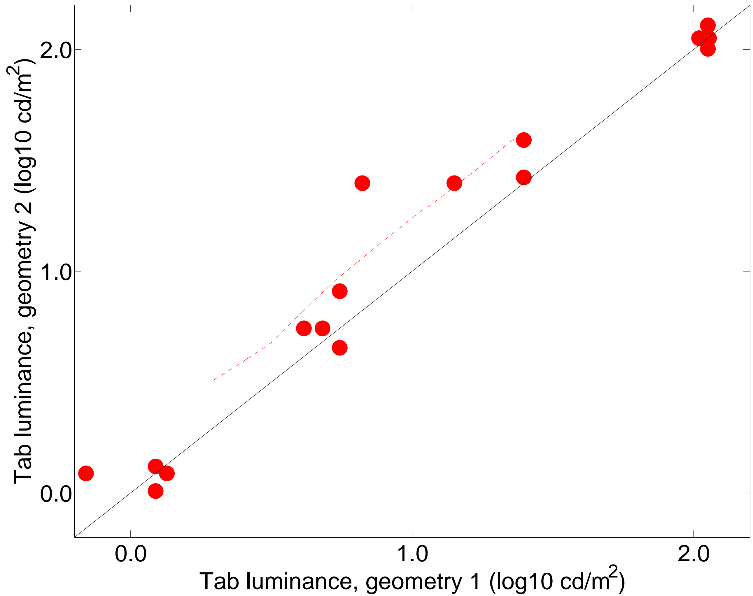
Obs A5, PSEs for binocular condition
